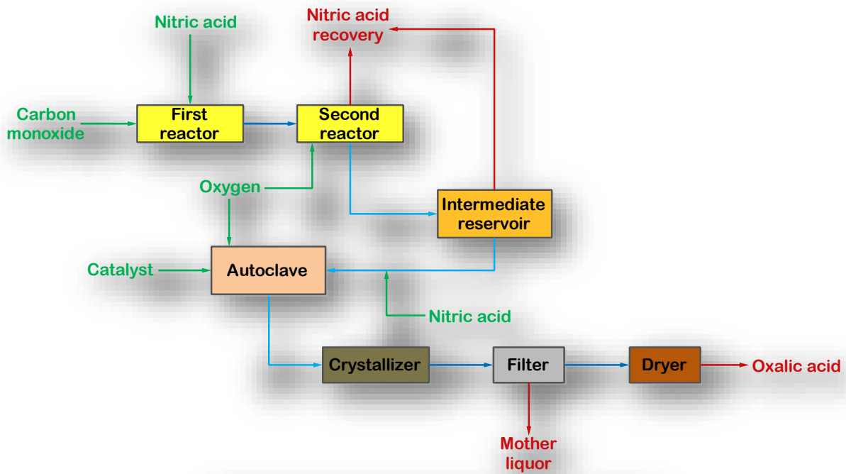
Figure: Manufacture of Oxalic acid from Propylene
